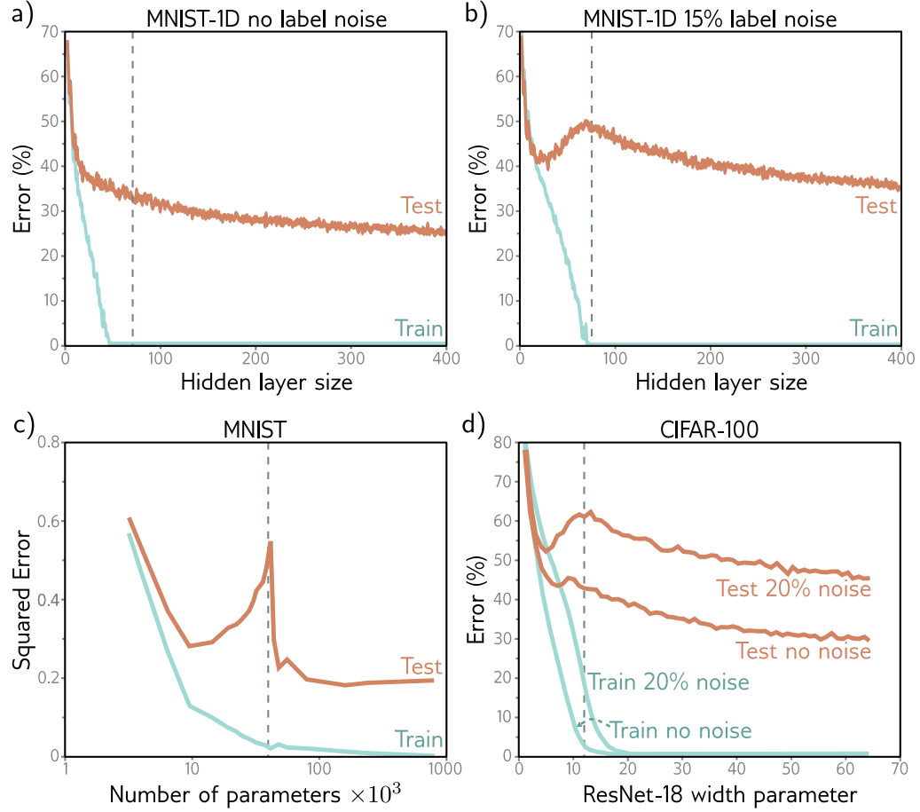
Figure 8.10 Double descent. a) Training and test error on MNIST-1D for a two-hidden layer network as we increase the number of hidden units (and hence parameters) in each layer. The training error decreases to zero as the number of parameters approaches the number of training examples (vertical dashed line). The test error does not show the expected bias-variance trade-off but continues to decrease even after the model has memorized the dataset. b) The same experiment is repeated with noisier training data. Again, the training error reduces to zero, although it now takes almost as many parameters as training points to memorize the dataset. The test error shows the predicted bias/variance trade-off; it decreases as the capacity increases but then increases again as we near the point where the training data is exactly memorized. However, it subsequently decreases again and ultimately reaches a better performance level. This is known as double descent. Depending on the loss function, the model, and the amount of noise in the data, the double descent pattern can be seen to a greater or lesser degree across many datasets. c) Results on MNIST (without label noise) with shallow neural network from Belkin et al. (2019). d) Results on CIFAR-100 with ResNet18 network (see chapter 11) from Nakkiran et al. (2021). See original papers for details.
